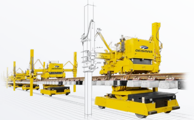
PEM-LEM | Laying solution for track, turnouts, switches and crossings
