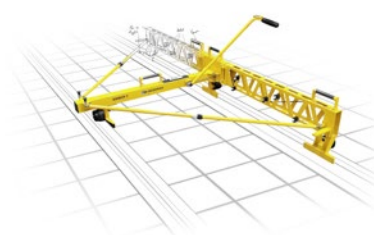
TRACK GEOMETRY AND VERSINE MEASURING AND RECORDING TROLLEY
