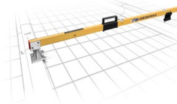
DIGITAL TRACK GAUGE FOR TRACK AND SWITCH GEOMETRY MEASUREMENT
