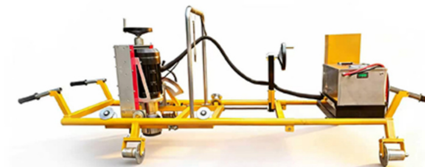
LK-LDDM-I BATTERY TURNOUT VERTICAL GRINDING MACHINE
