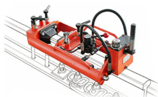
HWS-II HYDRAULIC WELD TRIM- MER MANUAL TYPE
